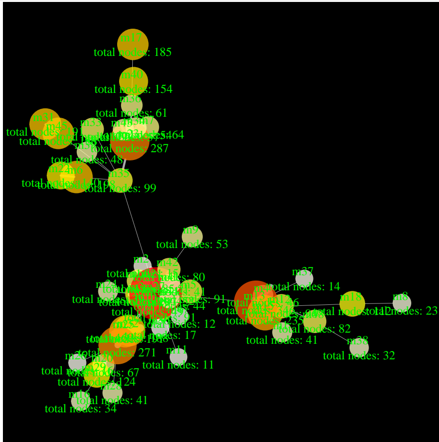
Figure 6: Abstract modular view of artificial network 2 ( |V| = 5,000, |E| = 23,878 ) emphasizing the labels of each module, the size of each module and the total number of connections between modules
