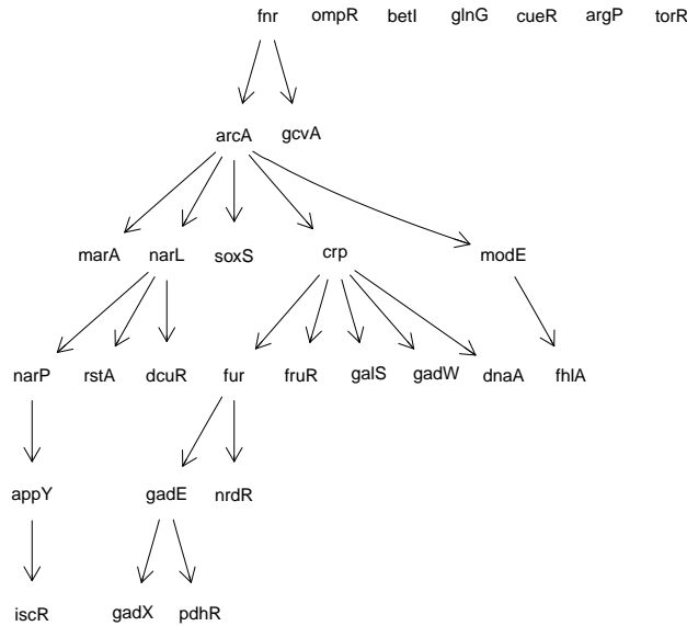
Figure 2: Inferred network between active TFs.
