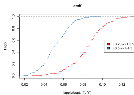
Figure 45: Distribution of bootstrap-resampled optimal costs ("disorder penalties").
