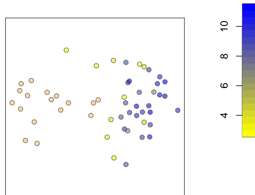
Figure 24: MDS plot of the E3.25 wild type (yellow–blue) and FGF4-KO (orange) samples. The yellow–blue colour scale represents the FGF4 expression level, as indicated in the colour bar.
