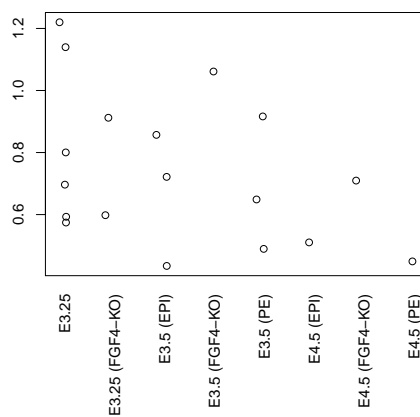
Figure 26: Variability of different groups of samples. The groups were defined by sample Group and ScanDate (see definition of varGroups above). Variability was measured by the median (across the 100 top variable genes) of the median absolute deviation across samples.
