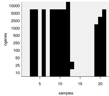
Figure 7: The influence of the parameter ngenes on the clustering result. Each of the 22 samples corresponds to a column of the matrix, the rows of the matrix correspond to different choices for ngenes . Cluster membership is indicated by the colour code (light gray vs black). For most samples, cluster membership is consistent throughout the range of ngenes from 10 to 1000. ngenes = 1000 is used for subsequent analyses.
