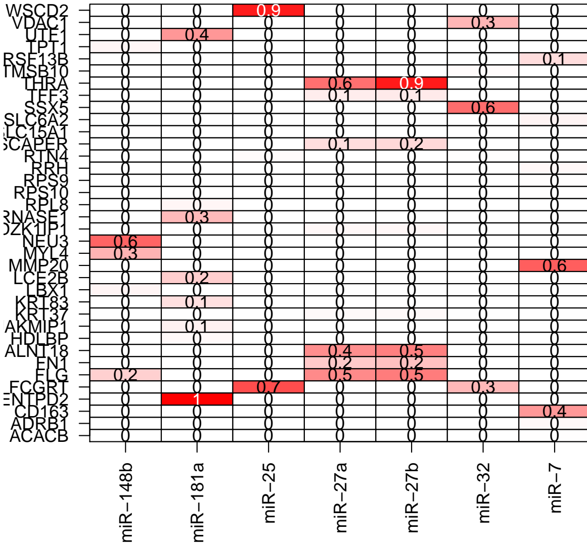
Figure 3: ProMISe generated from Section 4. Probabilities are displayed in the cells. The intensity of the red color corresponds to the magnitude of the probabilities (i.e. the higher the probability the more red).
