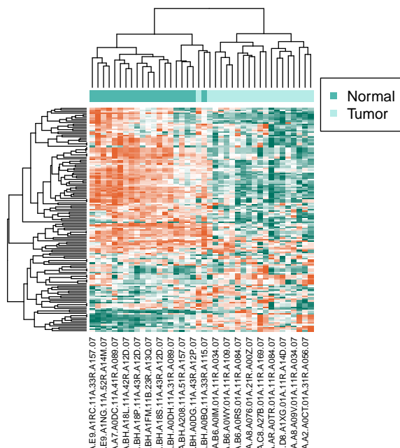
Figure 7: Heatmap plots with variable clustering
