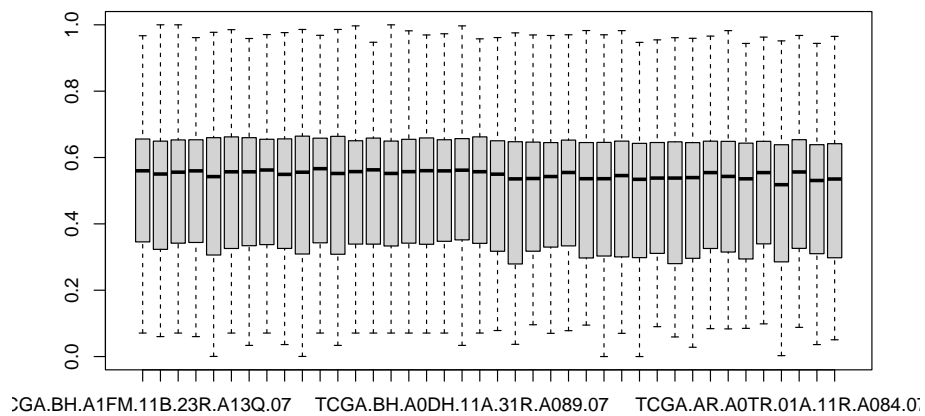
Figure 5: BRCA data after truncating by percentil 0.95
