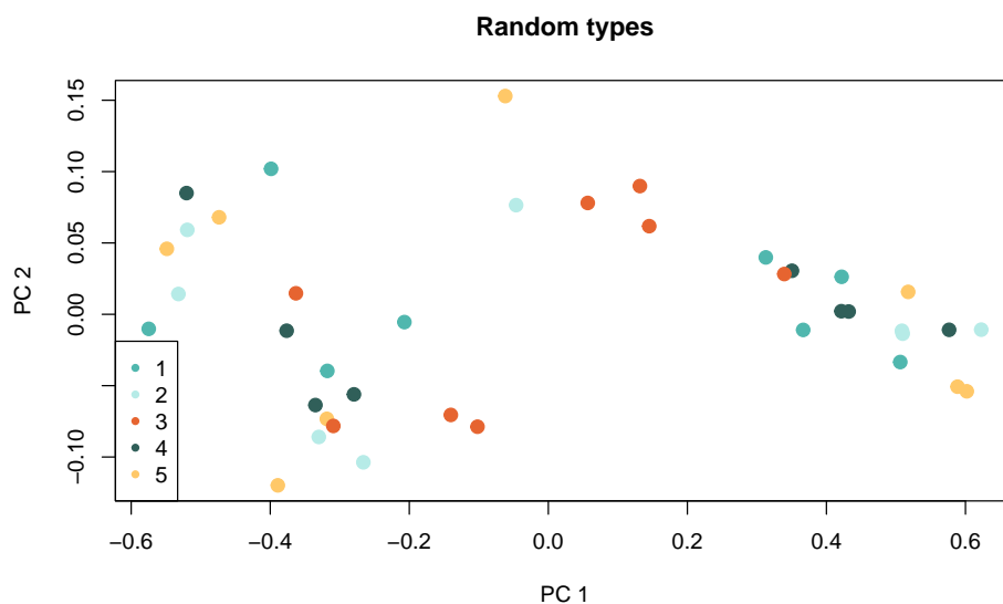
Figure 10: PCA plot with 5 random colors
