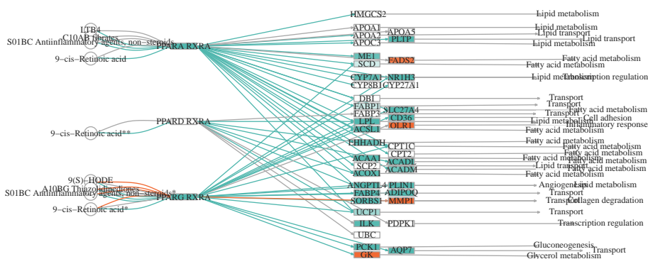
Figure 14: Pathway comparison plot with node colors: 'hipathia'
