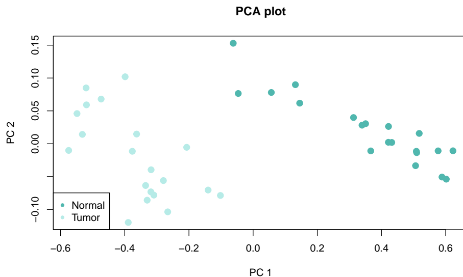
Figure 9: PCA plot
