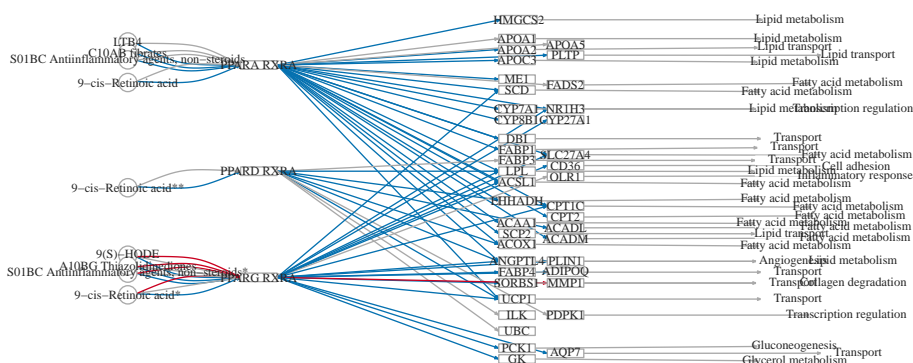
Figure 12: Pathway comparison plot without node colors
