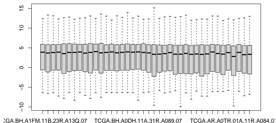
Figure 1: BRCA data before scaling
