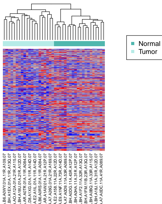
Figure 6: Heatmap plot
