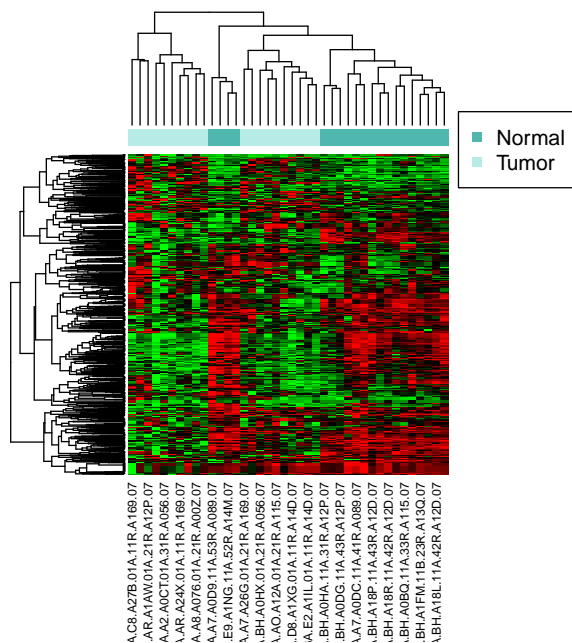
Figure 8: Different colors of heatmaps: 'redgreen'
