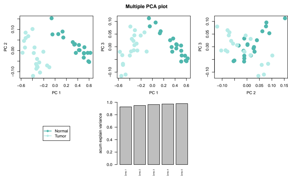
Figure 11: Multiple PCA plot with accumulated explained variance
