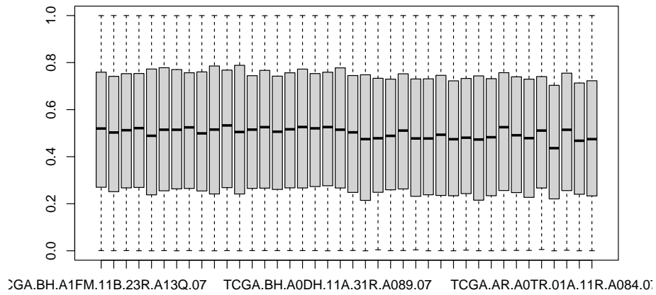
Figure 4: BRCA data after normalizing by percentil
