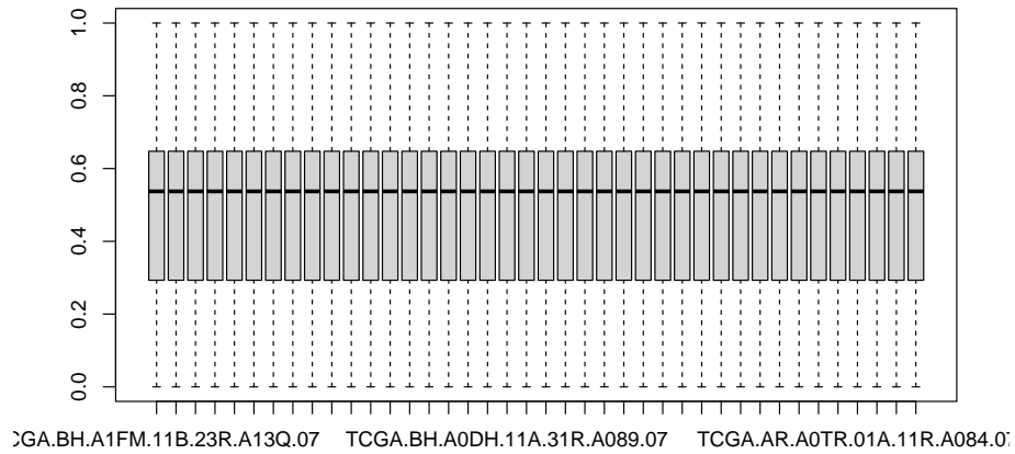
Figure 3: BRCA data after a Quantiles normalization
