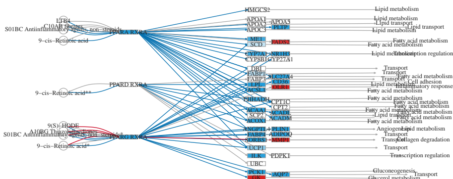
Figure 13: Pathway comparison plot with node colors: 'classic'
