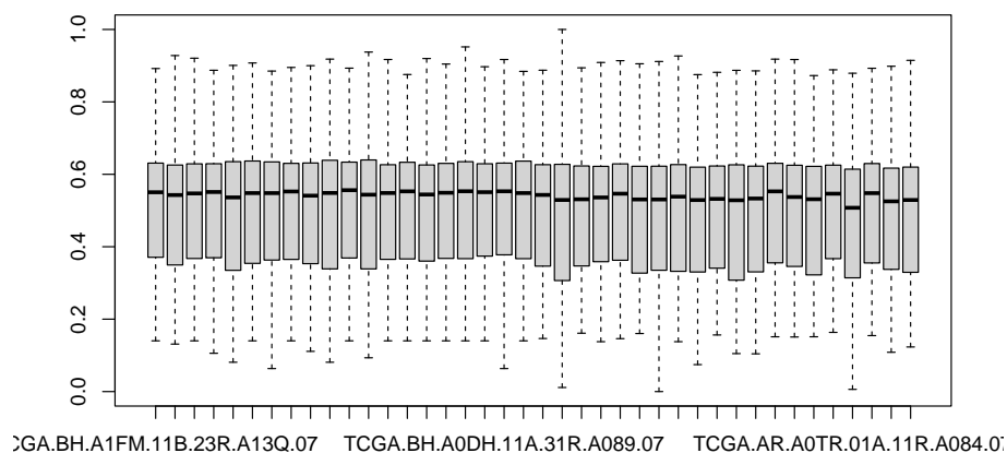
Figure 2: BRCA data after scaling
