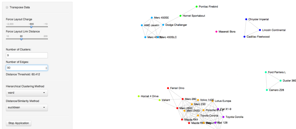
Figure 33: simplenet
