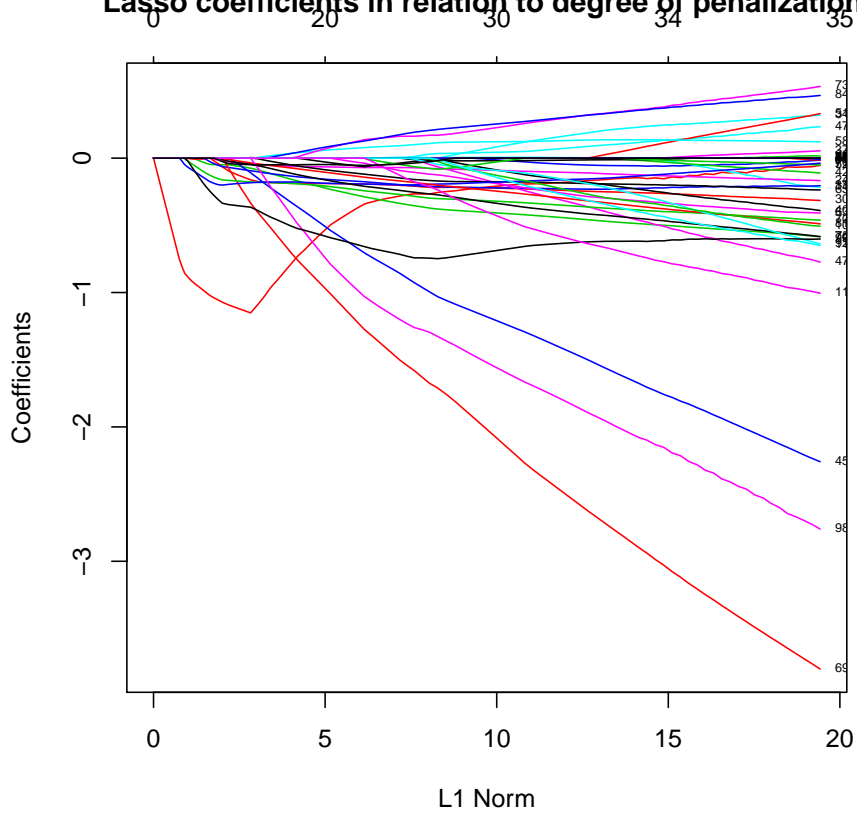
Lasso coefficients in relation to degree of penalization.
