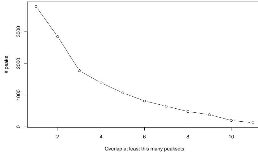
Figure 13: Overlap rate plot. Shows how the number of overlapping peaks decreases as the overlap criteria becomes more stringent. X axis shows the number of peaksets in which the site is identified, while the Y axis shows the number of overlapping sites. Generated by plotting the result of: dba.overlap(tamoxifen,mode=DBA_OLAP_RATE)
