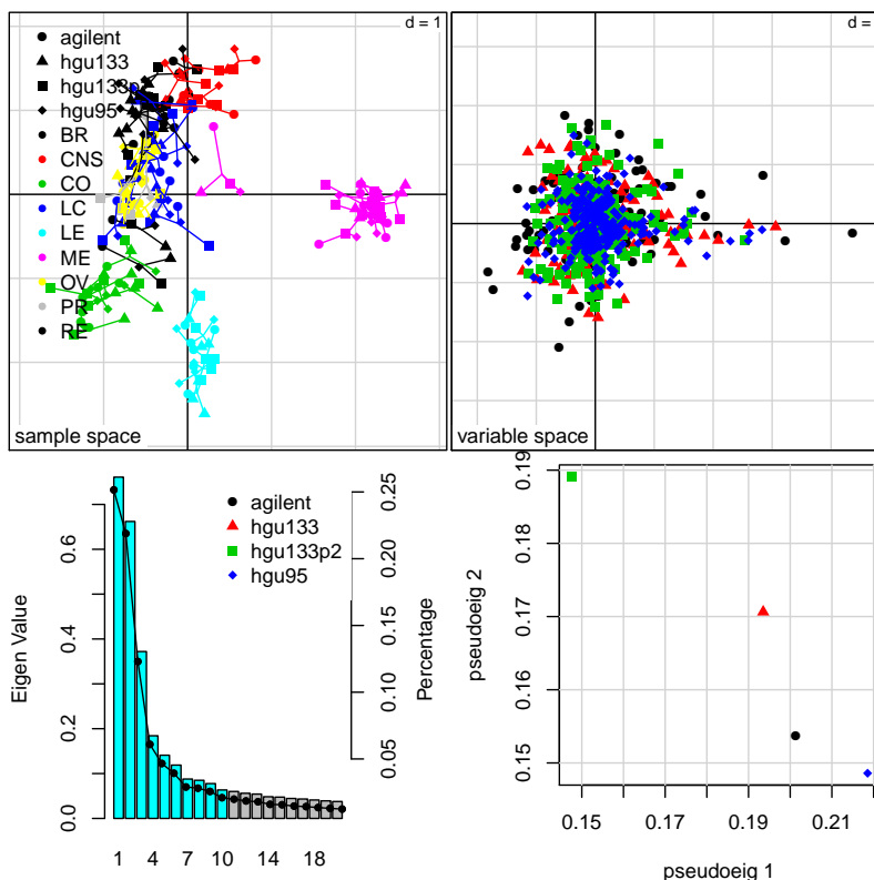
Figure 2: The MCI plot of NCI-60 data
