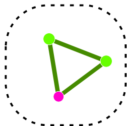
module15 (p.value=9.64e-03)
