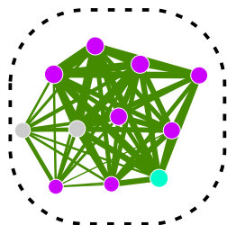
module11 (p.value=6.90e-03)
