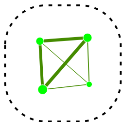
module10 (p.value=6.19e-03)
