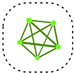
module5 (p.value=1.79e-03)
