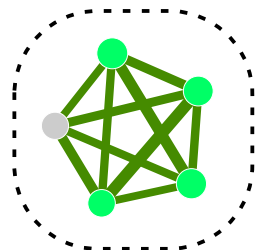
module12 (p.value=7.72e-03)
