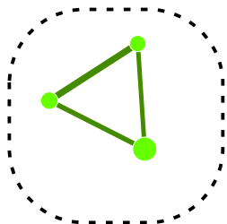
module14 (p.value=8.79e-03)
