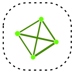
module7 (p.value=4.17e-03)
