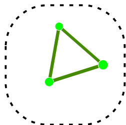
module7 (p.value=4.17e-03)
