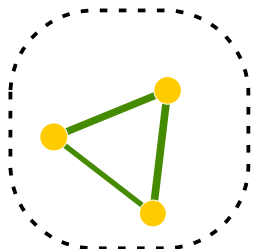
module5 (p.value=1.79e-03)
